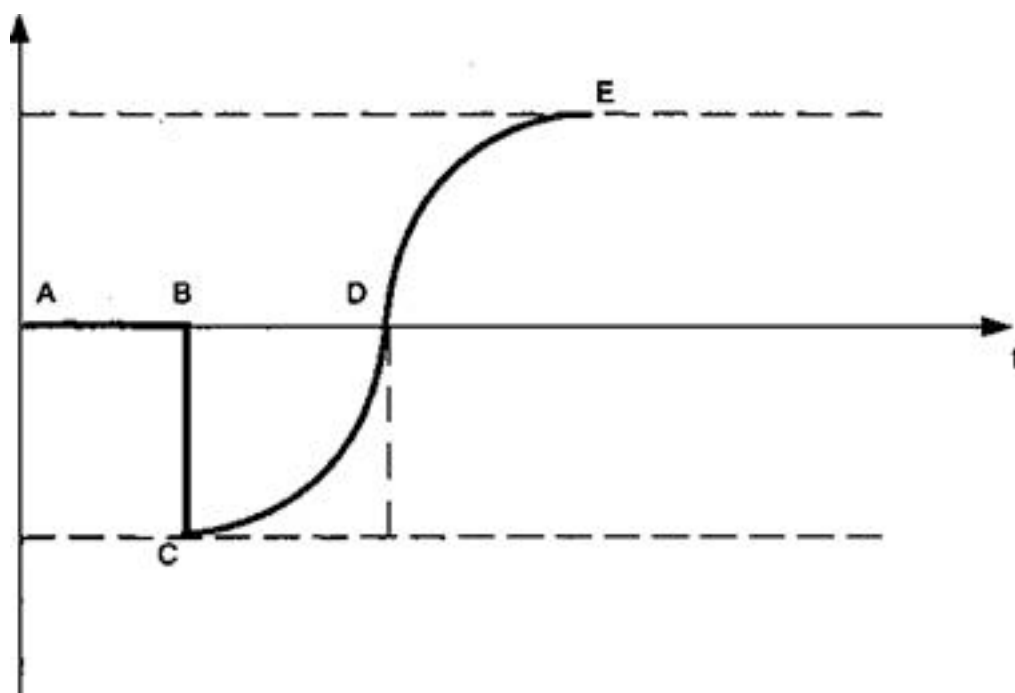
Figure 17.3. J-curve
