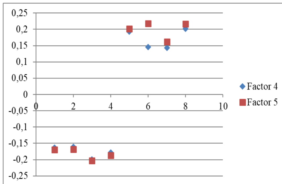
Figure 1. Factor Loading. Factor 4 vs Factor 5. Rotation. Unrotated. Extraction: Principal component Figure title
